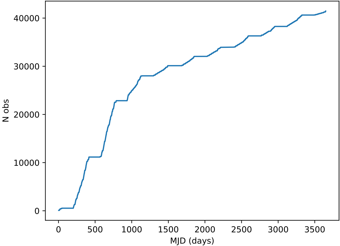
too_elab_heavy_r128_d3_gz_v3.4_10yrs all bands: DD:COSMOS Cumulative NVisits
