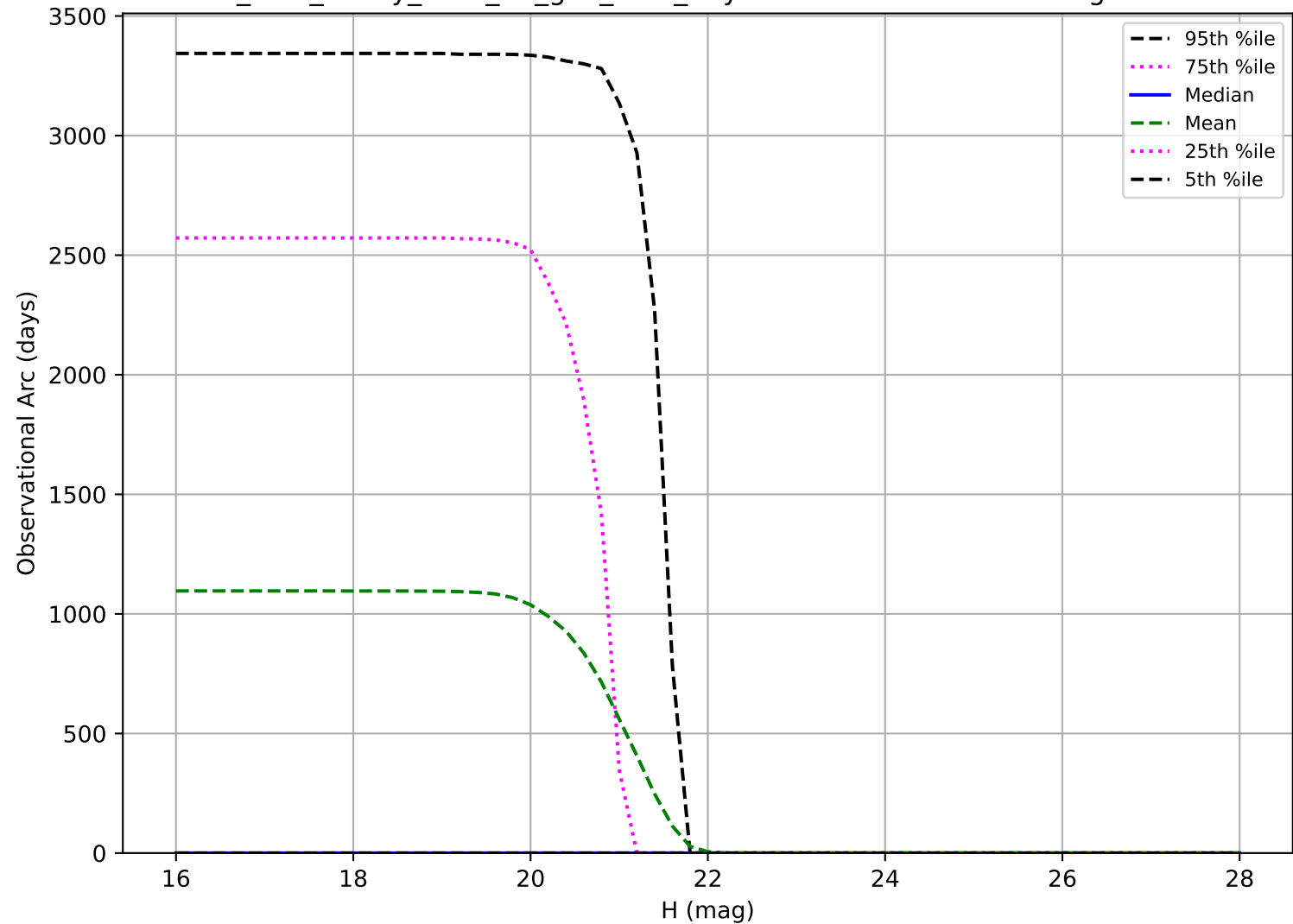
too_elab_heavy_r128_d3_griz_v3.4_10yrs: Observational Arc Length Vatira
