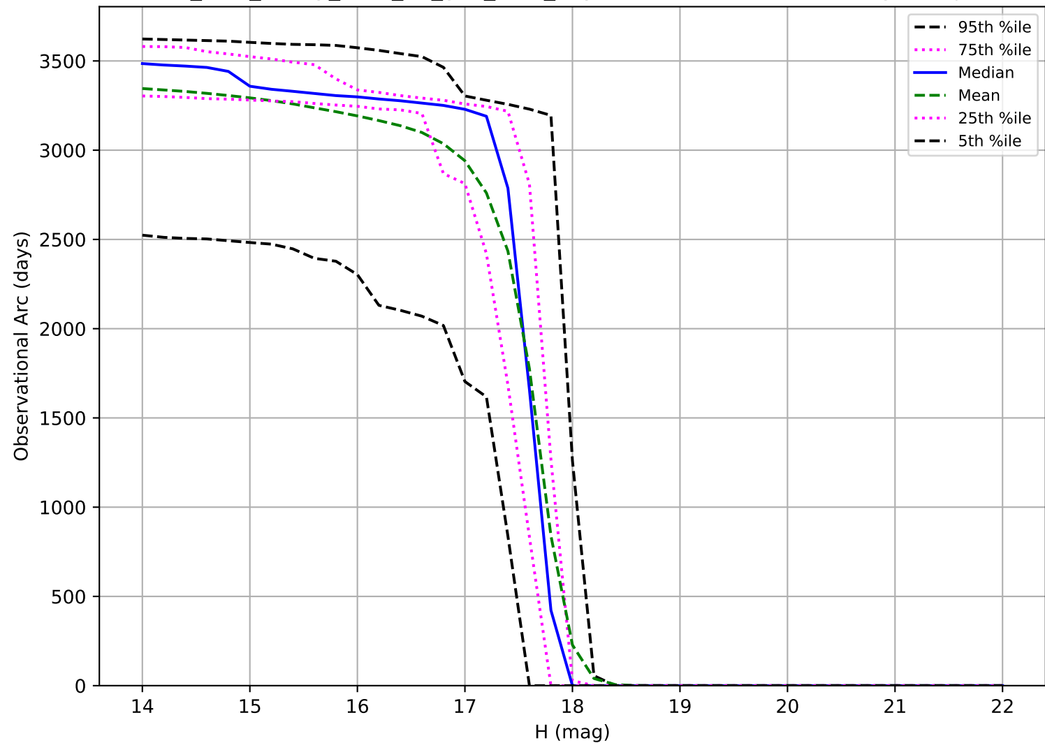
too_elab_heavy_r128_d3_griz_v3.4_10yrs: Observational Arc Length Trojan
