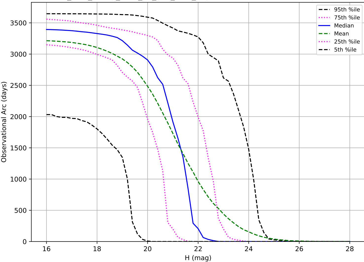
too_elab_heavy_r128_d3_griz_v3.4_10yrs: Observational Arc Length PHA
