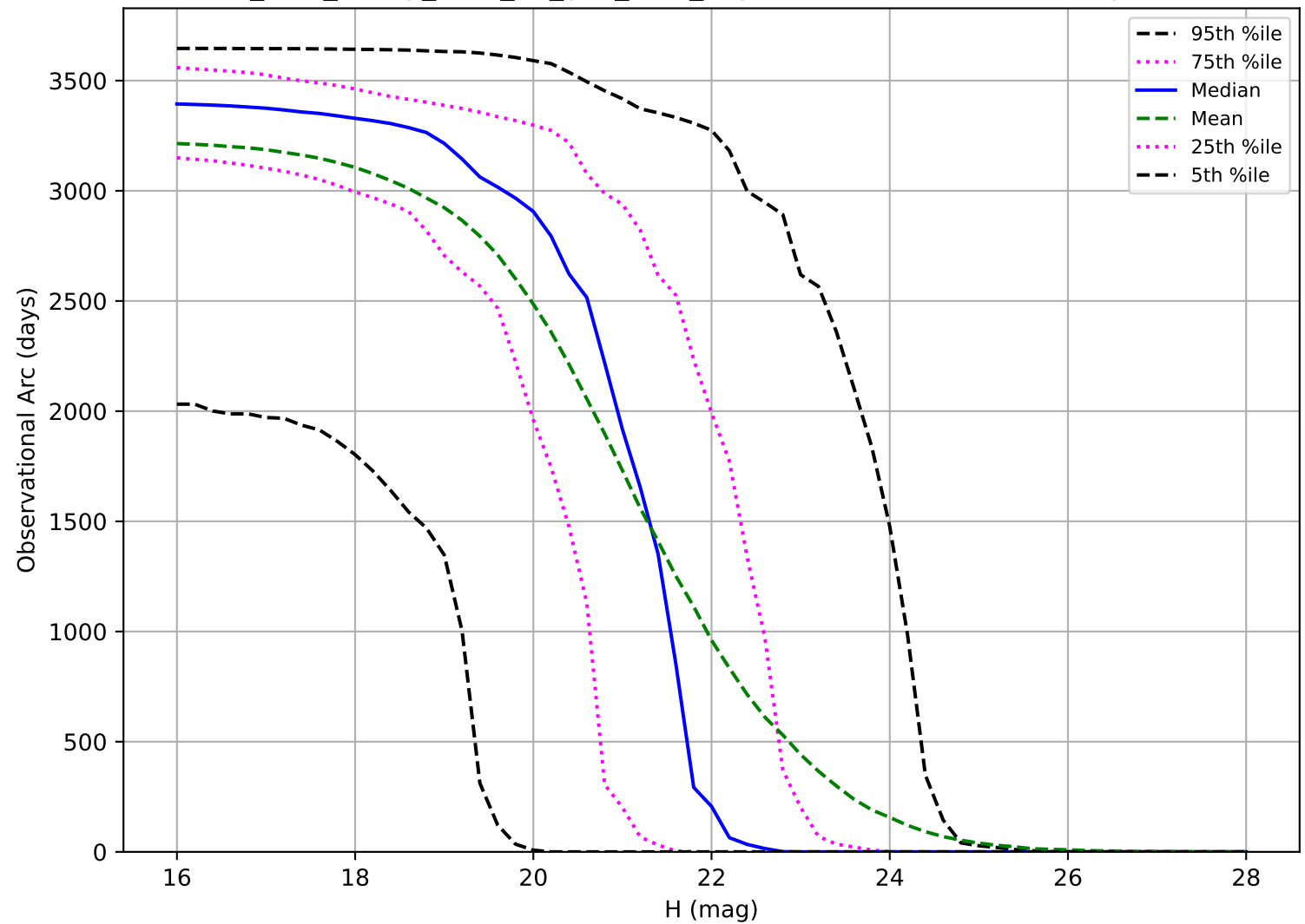
too_elab_heavy_r128_d3_griz_v3.4_10yrs: Observational Arc Length PHA
