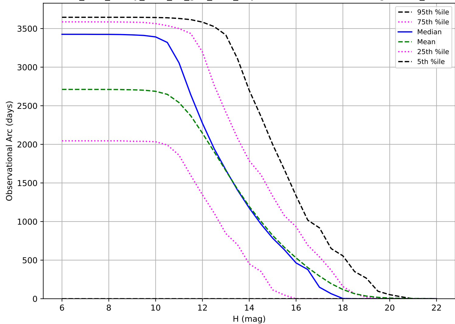
too_elab_heavy_r128_d3_griz_v3.4_10yrs: Observational Arc Length OCC_r5
