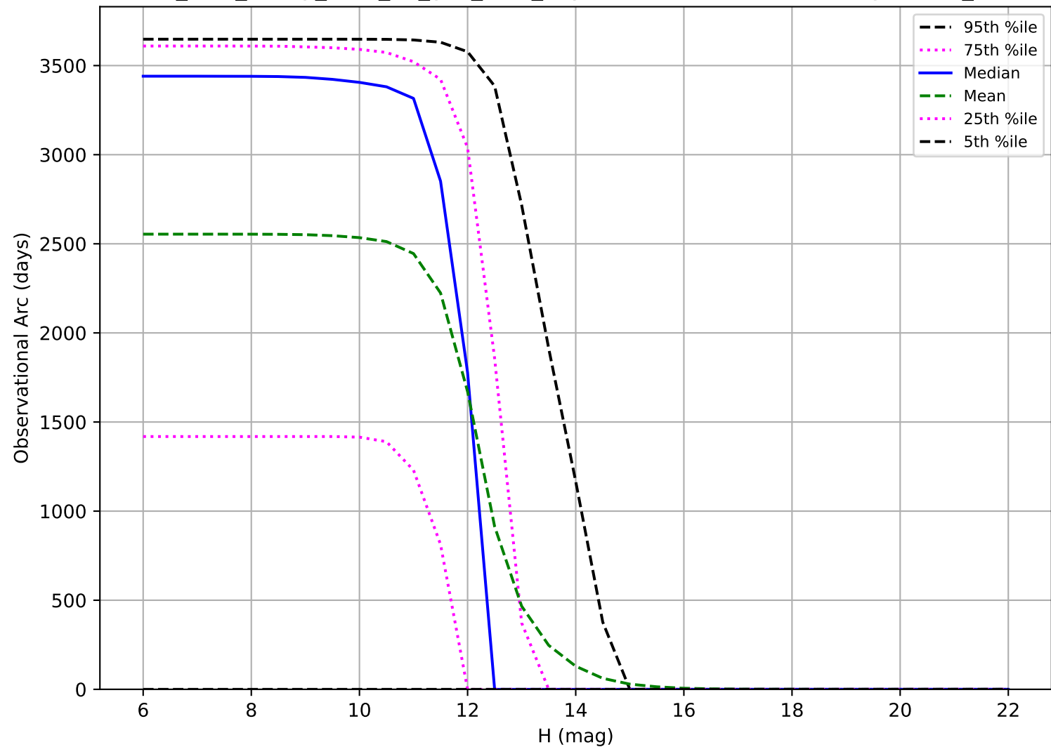
too_elab_heavy_r128_d3_griz_v3.4_10yrs: Observational Arc Length OCC_r20
