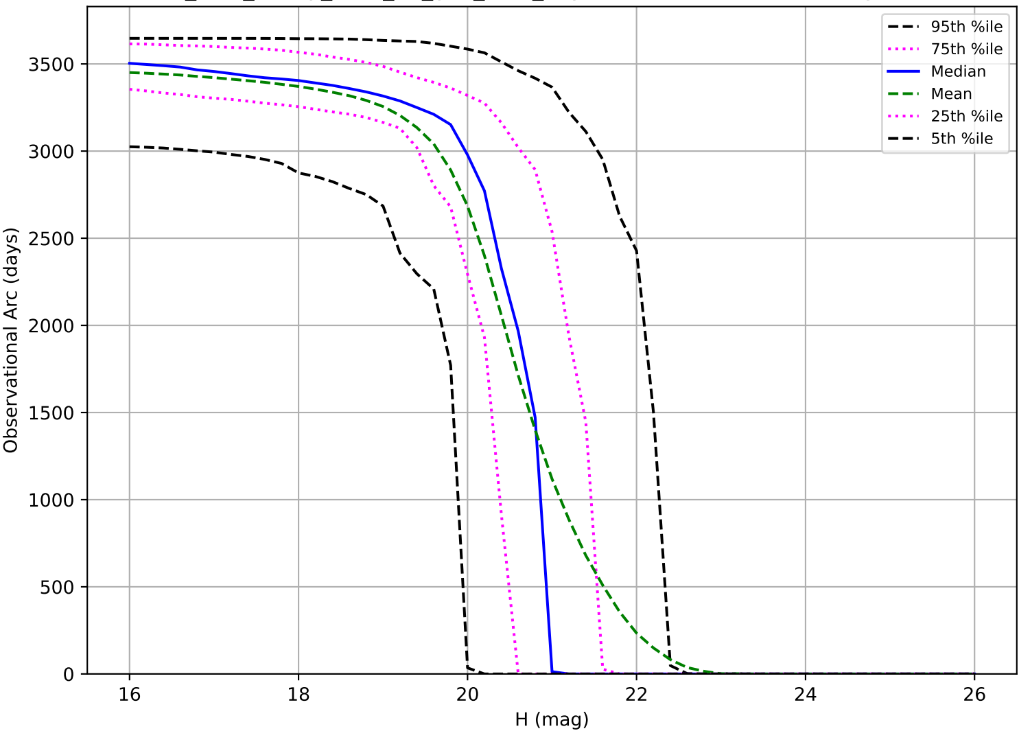
too_elab_heavy_r128_d3_griz_v3.4_10yrs: Observational Arc Length MBA
