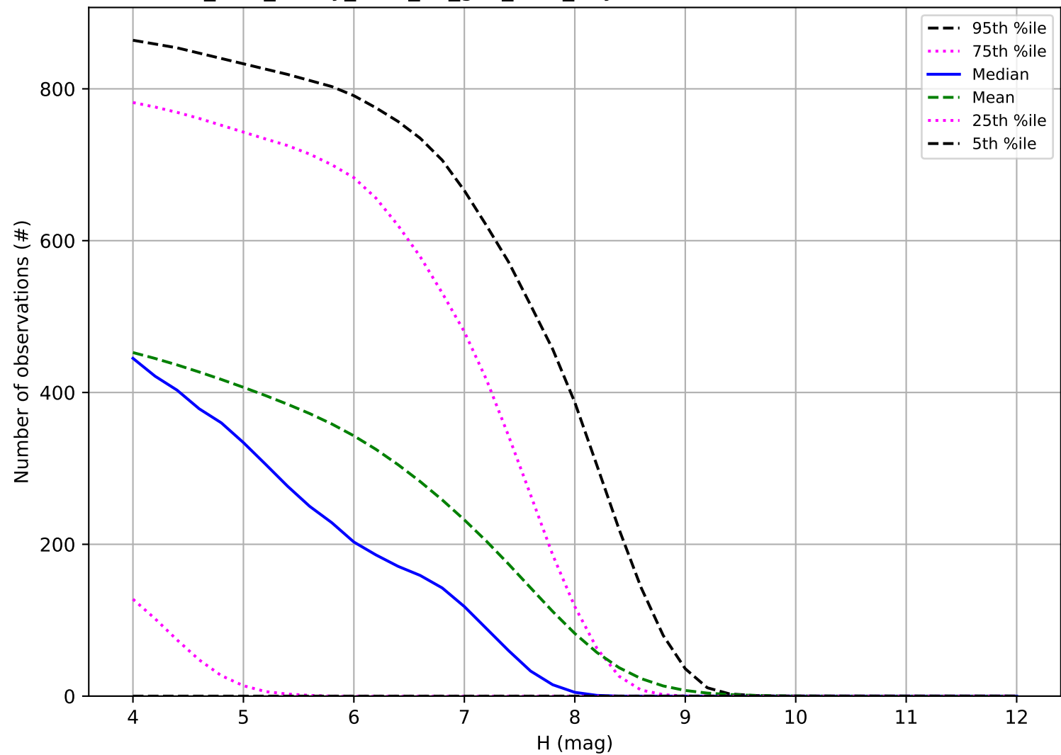
too_elab_heavy_r128_d3_griz_v3.4_10yrs: Number of observations TNO
