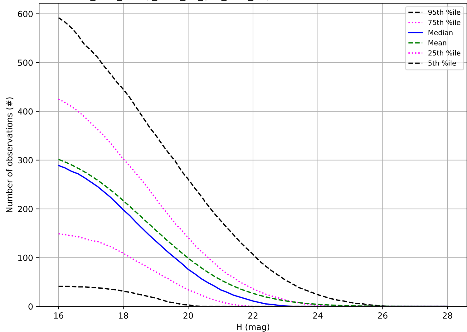
too_elab_heavy_r128_d3_griz_v3.4_10yrs: Number of observations PHA
