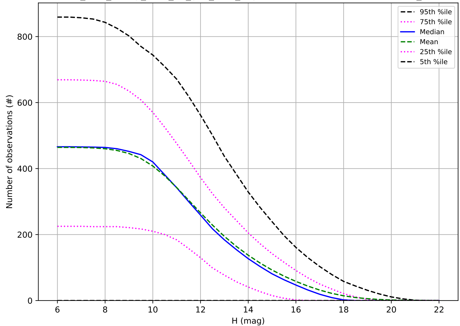
too_elab_heavy_r128_d3_griz_v3.4_10yrs: Number of observations OCC_r5
