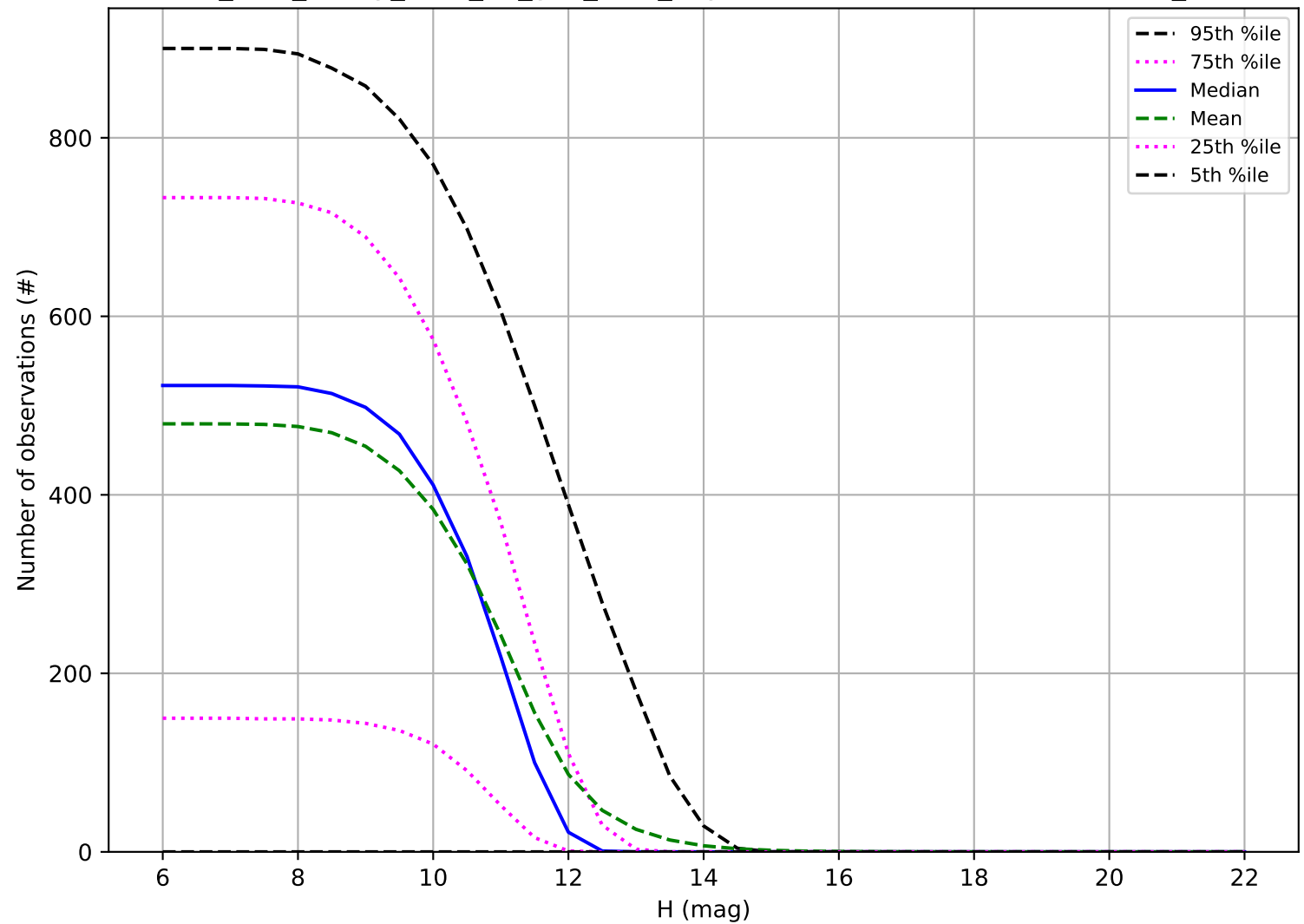
too_elab_heavy_r128_d3_griz_v3.4_10yrs: Number of observations OCC_r20
