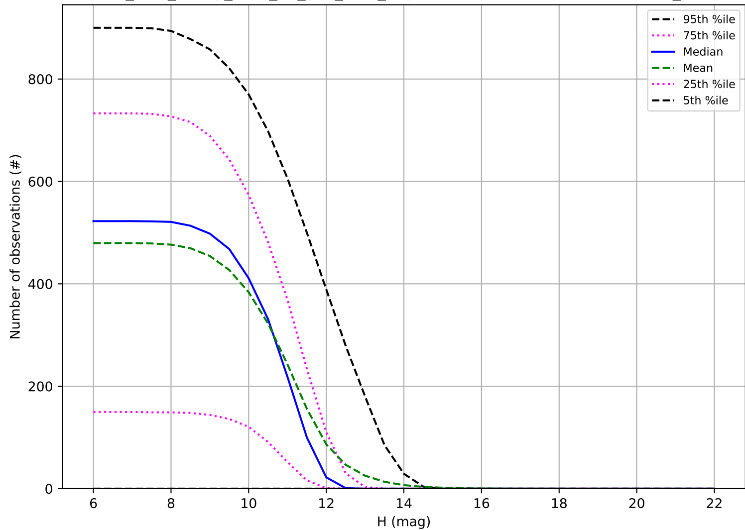
too_elab_heavy_r128_d3_griz_v3.4_10yrs: Number of observations OCC_r20
