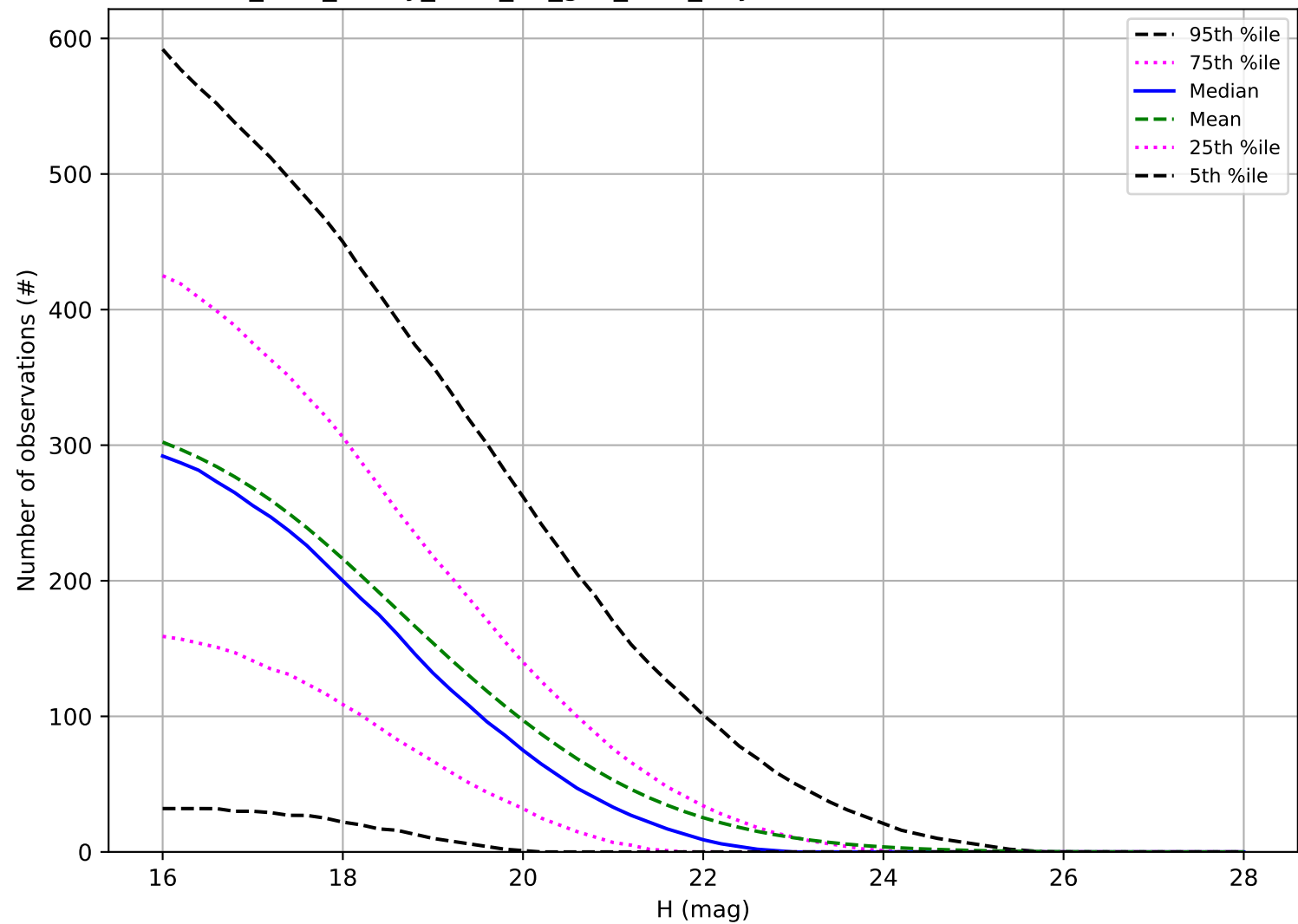
too_elab_heavy_r128_d3_griz_v3.4_10yrs: Number of observations NEO
