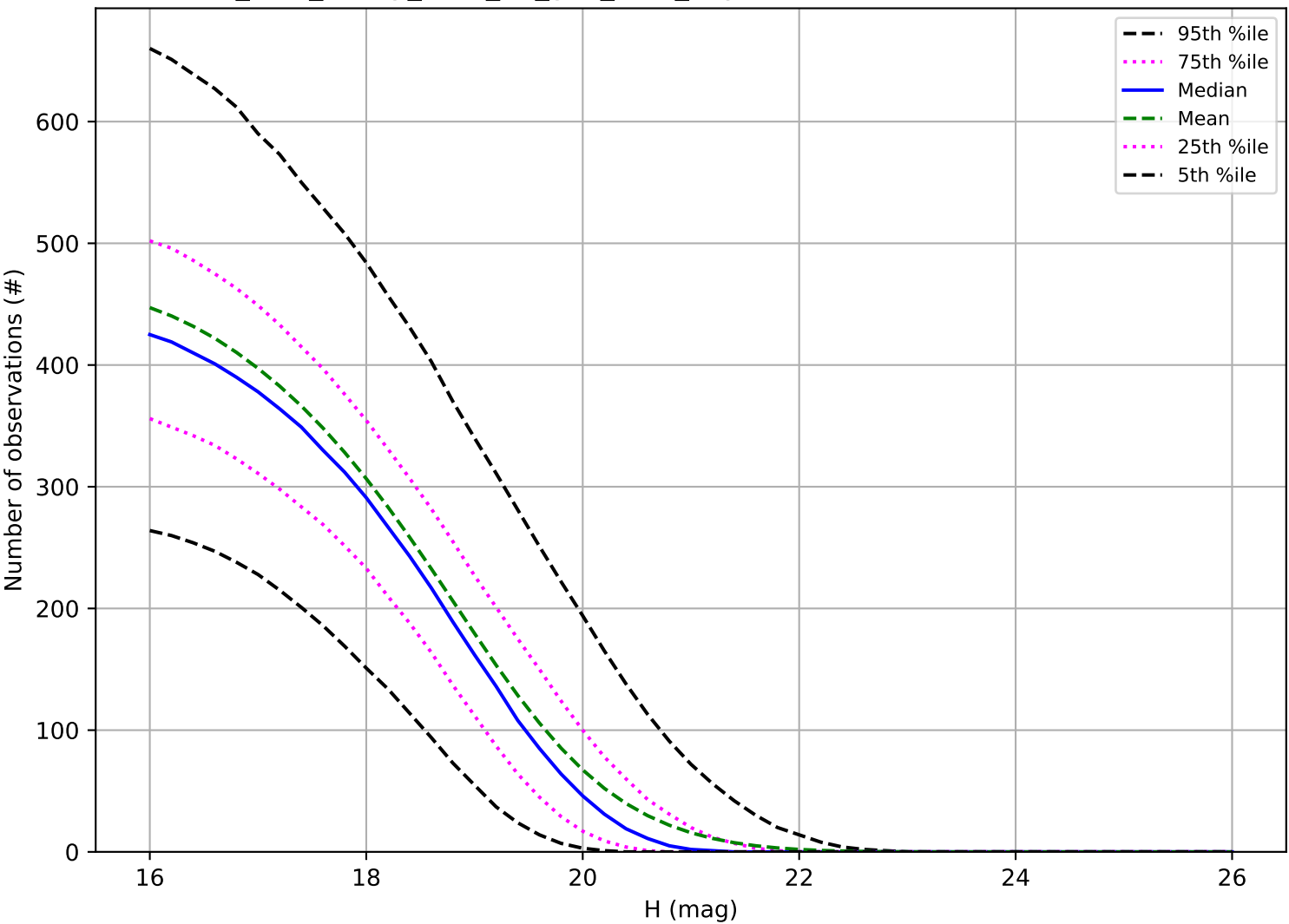
too_elab_heavy_r128_d3_griz_v3.4_10yrs: Number of observations MBA
