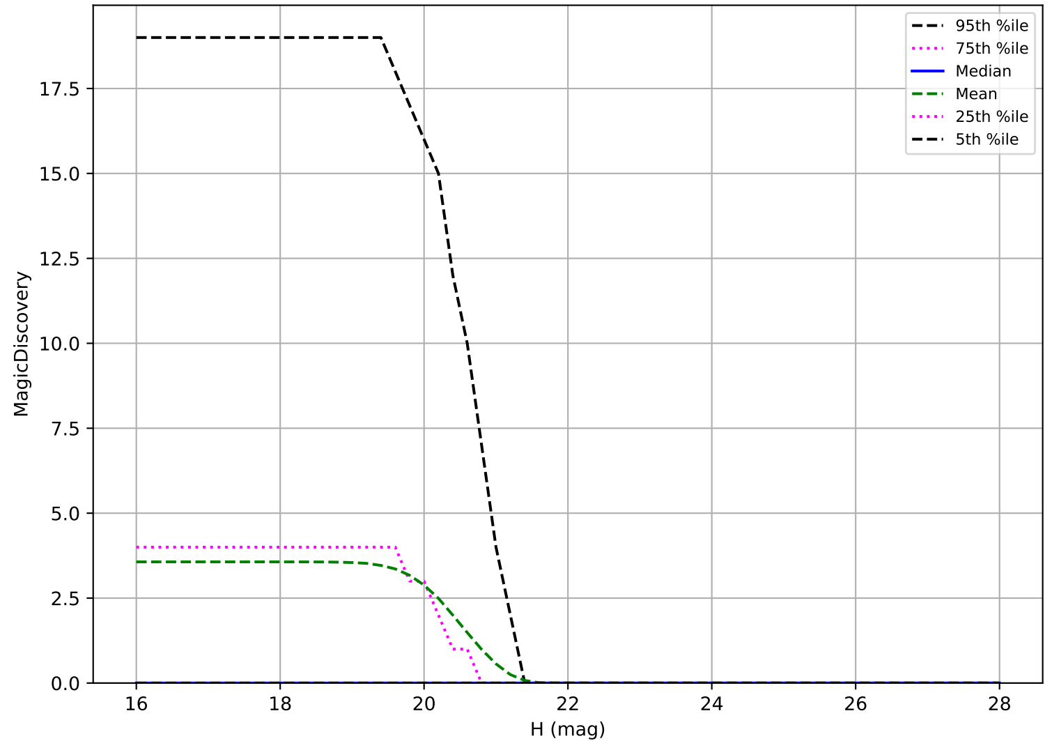
too_elab_heavy_r128_d3_griz_v3.4_10yrs: Vaira 6 detections in 60 nights detection loss
