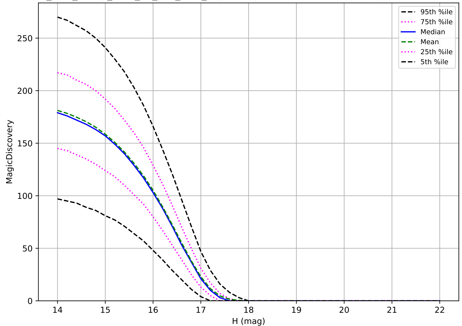
too_elab_heavy_r128_d3_griz_v3.4_10yrs: Trojan 6 detections in 60 nights detection loss
