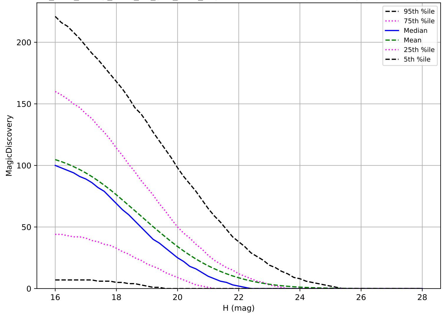
too_elab_heavy_r128_d3_griz_v3.4_10yrs: PHA 6 detections in 60 nights detection loss
