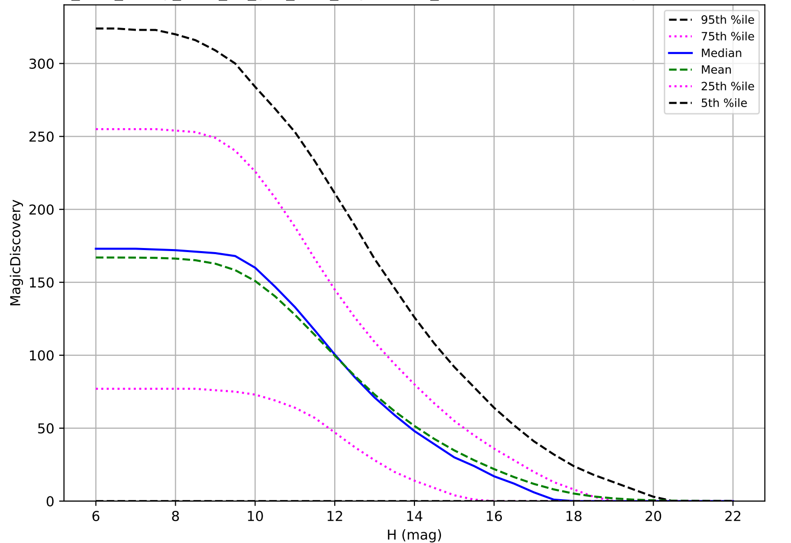
too_elab_heavy_r128_d3_griz_v3.4_10yrs: OCC_r5 6 detections in 60 nights detection loss
