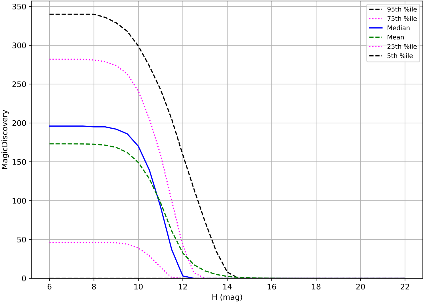
too_elab_heavy_r128_d3_griz_v3.4_10yrs: OCC_r20 6 detections in 60 nights detection loss
