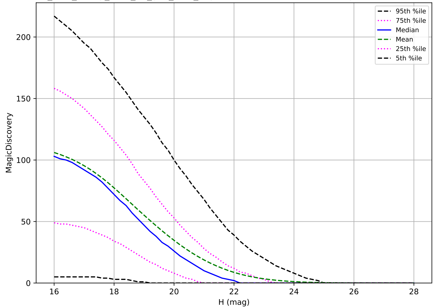
too_elab_heavy_r128_d3_griz_v3.4_10yrs: NEO 6 detections in 60 nights detection loss
