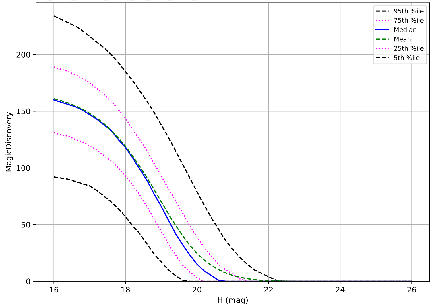
too_elab_heavy_r128_d3_griz_v3.4_10yrs: MBA 6 detections in 60 nights detection loss
