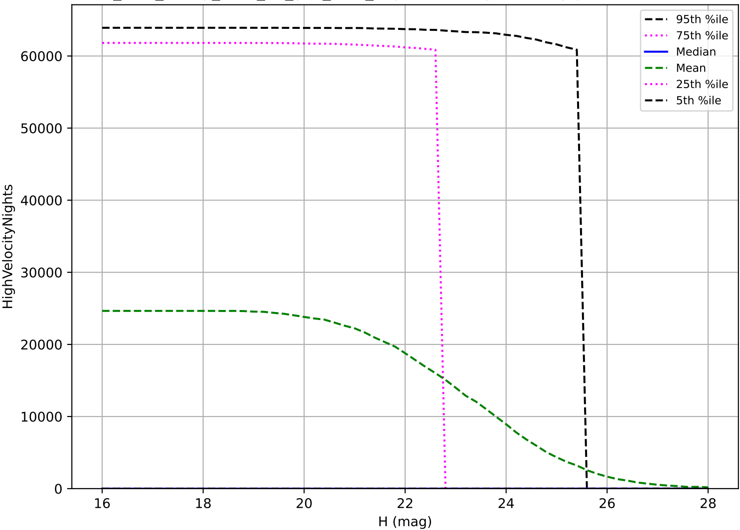
too_elab_heavy_r128_d3_griz_v3.4_10yrs: PHA High velocity pair detection loss
