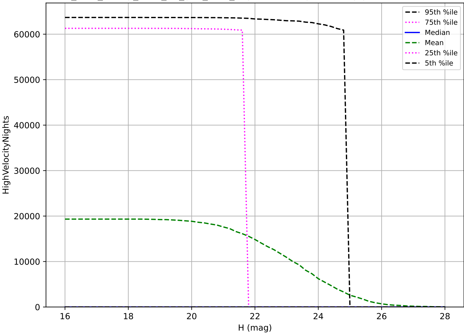
too_elab_heavy_r128_d3_griz_v3.4_10yrs: NEO High velocity pair detection loss
