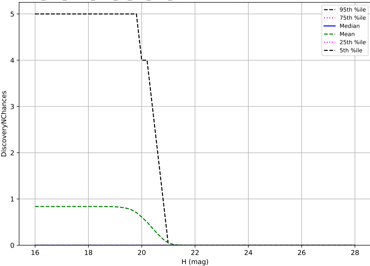
too_elab_heavy_r128_d3_griz_v3.4_10yrs: Vatira 3 pairs in 15 nights detection loss
