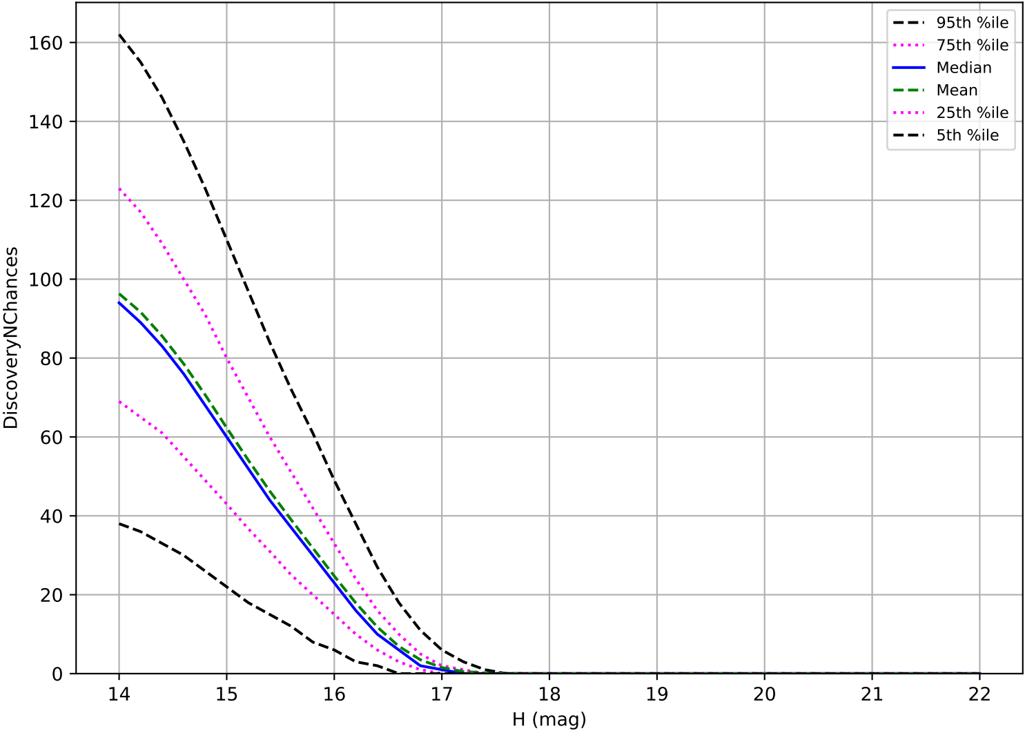
too_elab_heavy_r128_d3_griz_v3.4_10yrs: Trojan 3 pairs in 15 nights detection loss
