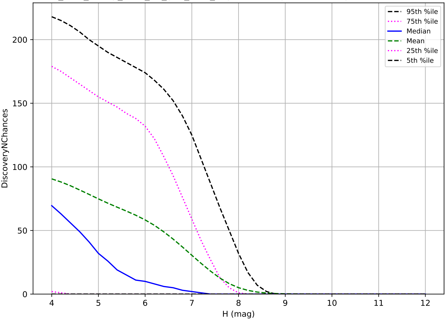
too_elab_heavy_r128_d3_griz_v3.4_10yrs: TNO 3 pairs in 15 nights detection loss
