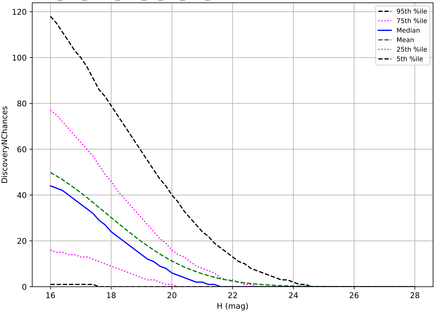
too_elab_heavy_r128_d3_griz_v3.4_10yrs: PHA 3 pairs in 15 nights detection loss
