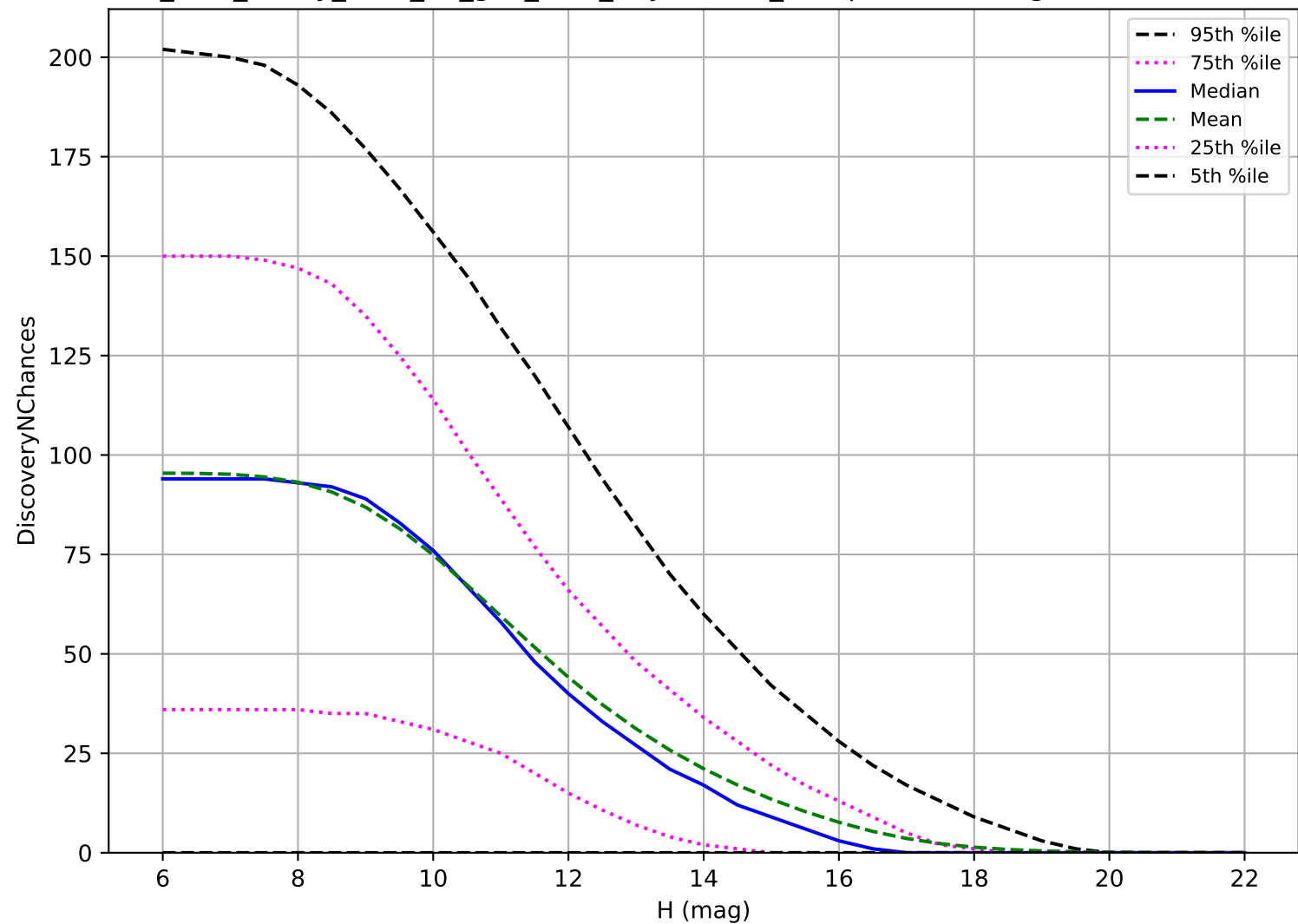
too_elab_heavy_r128_d3_griz_v3.4_10yrs: OCC_r5 3 pairs in 15 nights detection loss
