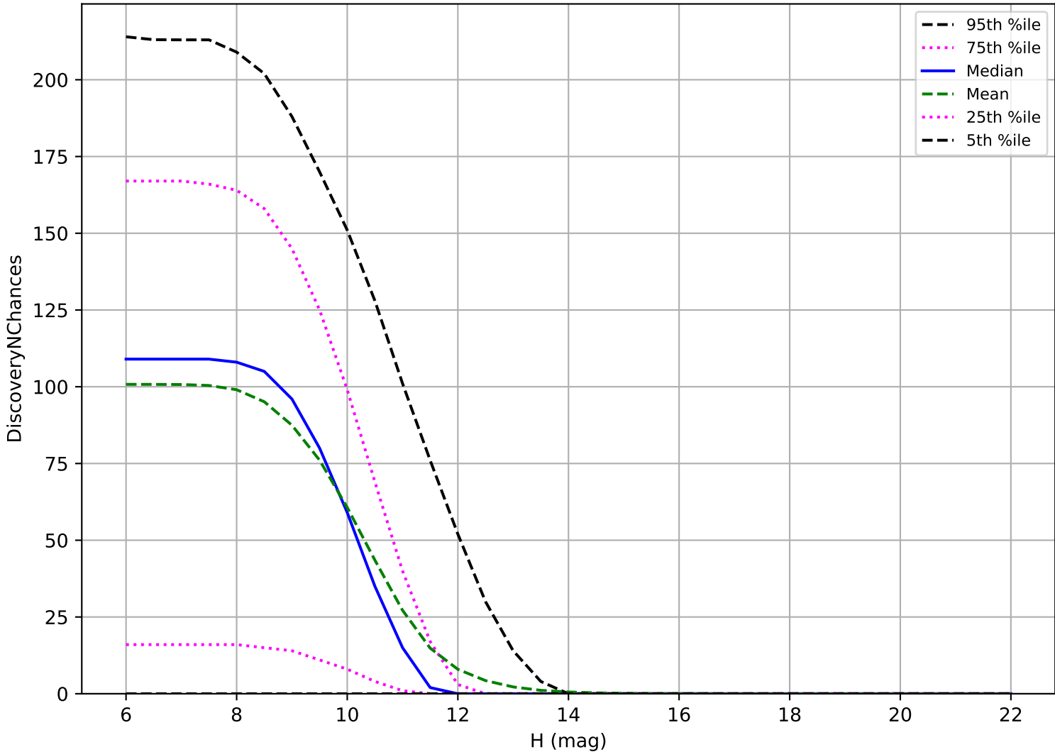
too_elab_heavy_r128_d3_griz_v3.4_10yrs: OCC_r20 3 pairs in 15 nights detection loss
