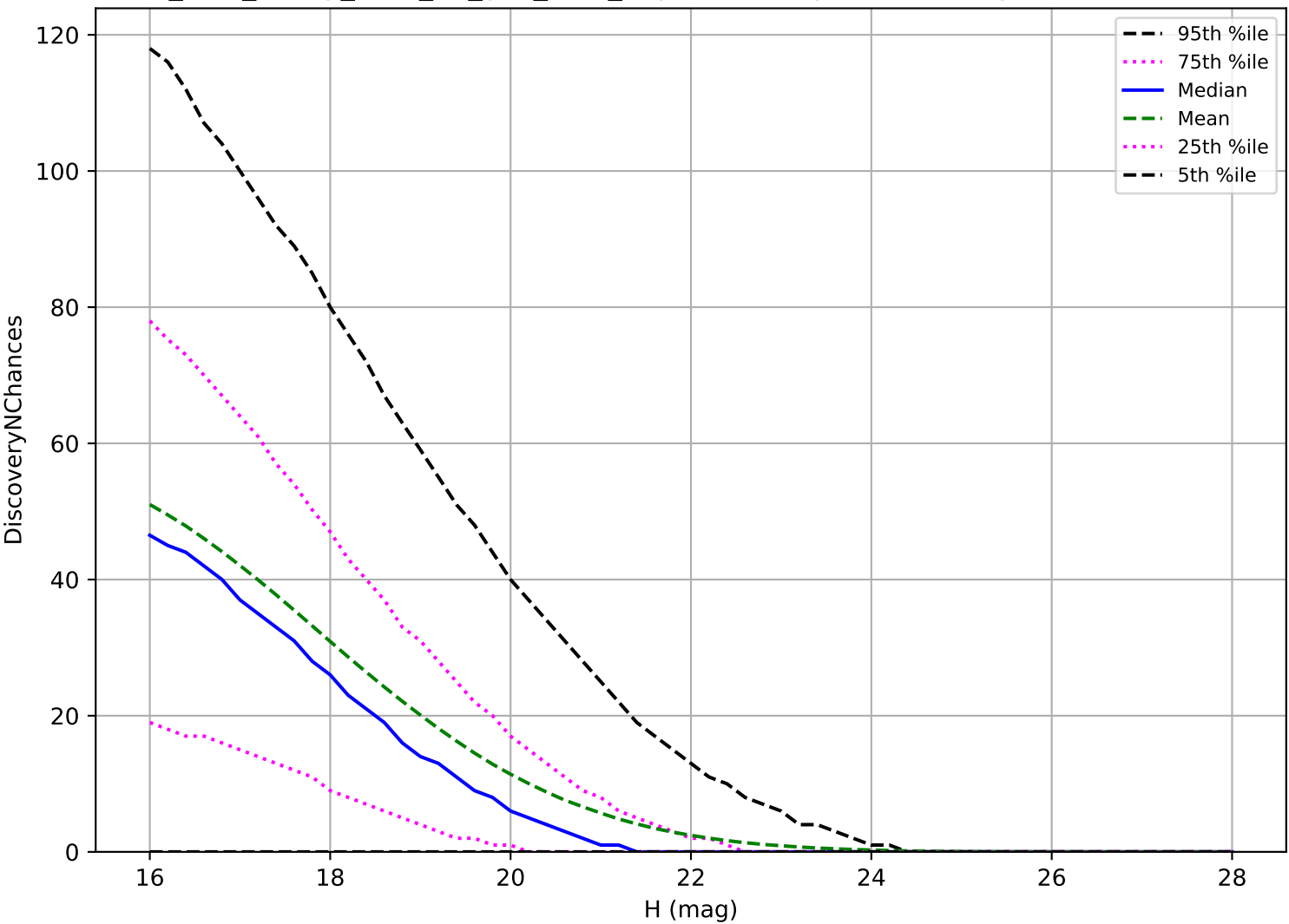
too_elab_heavy_r128_d3_griz_v3.4_10yrs: NEO 3 pairs in 15 nights detection loss
