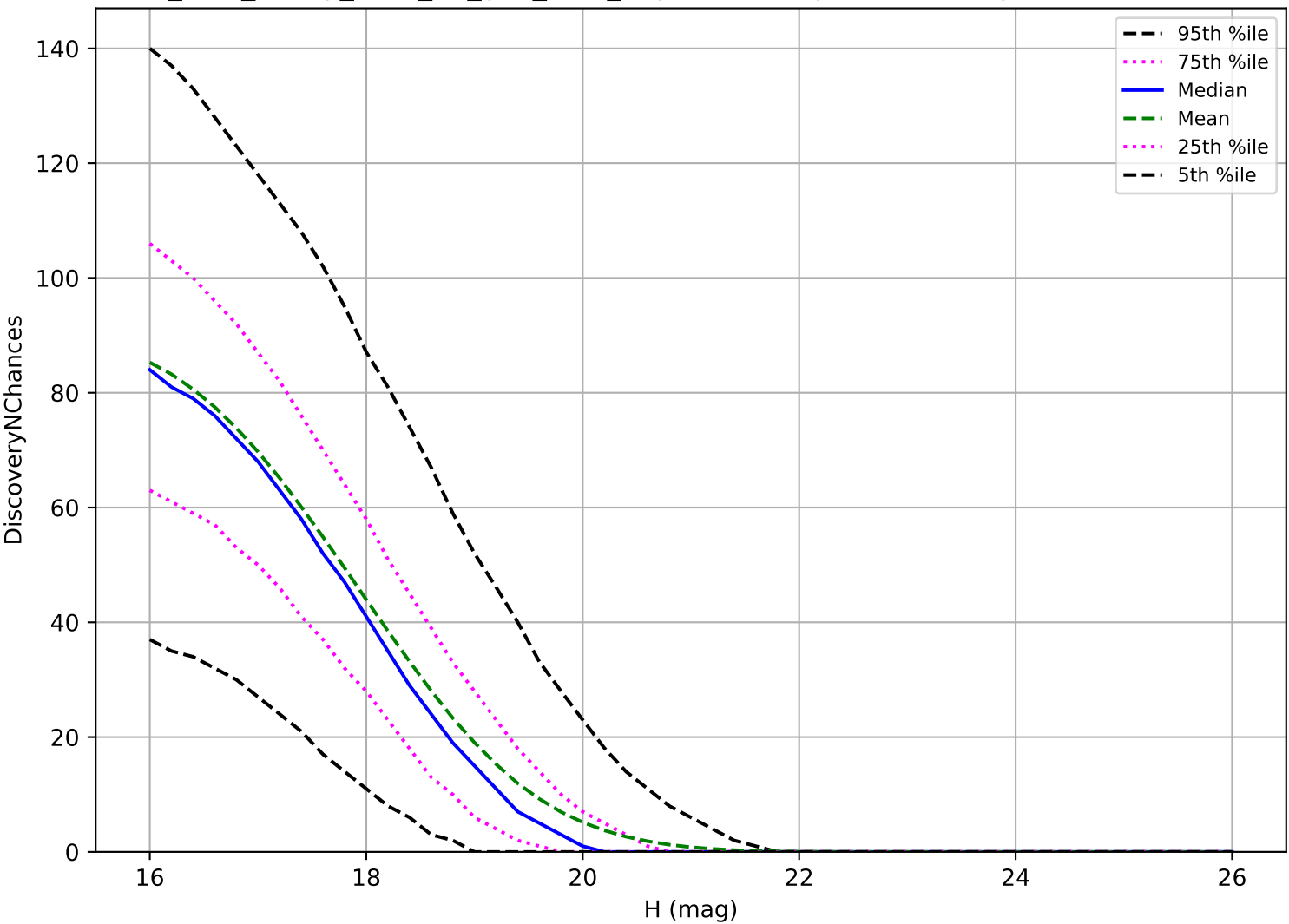
too_elab_heavy_r128_d3_griz_v3.4_10yrs: MBA 3 pairs in 15 nights detection loss
