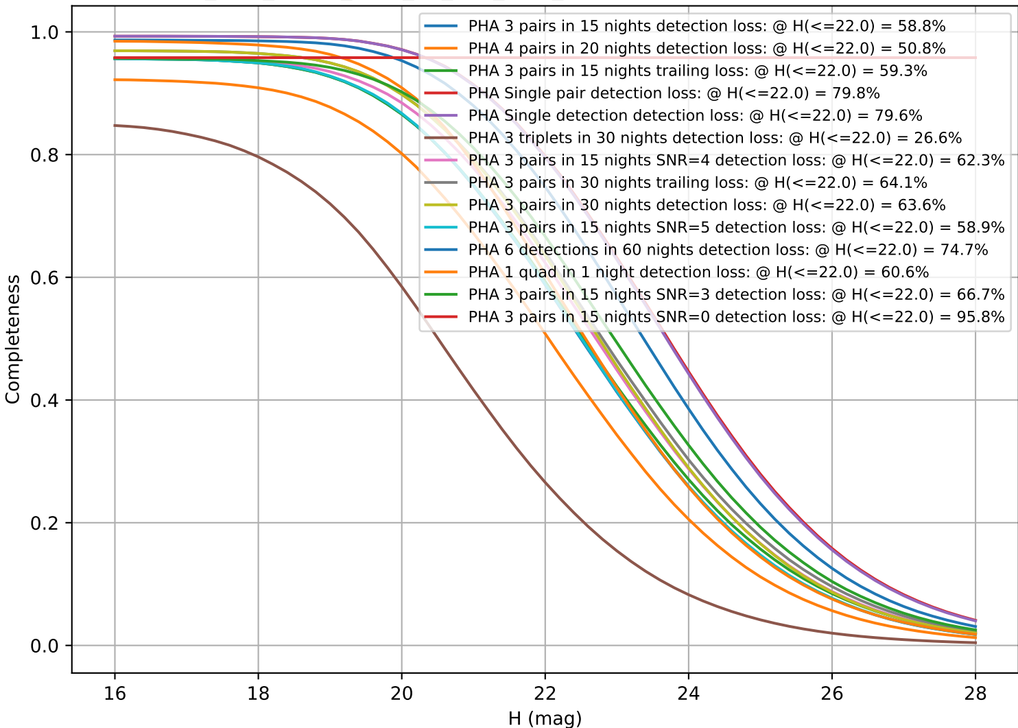
too_elab_heavy_r128_d3_griz_v3.4_10yrs: CumulativeCompleteness
