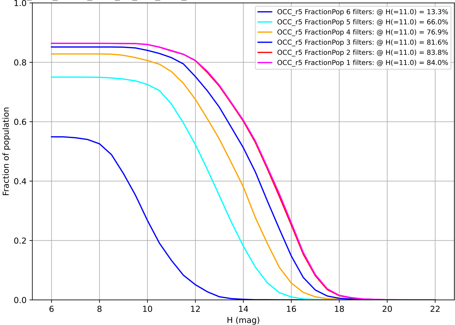
too_elab_heavy_r128_d3_griz_v3.4_10yrs: Fraction of population with colors in X filters OCC_r5
