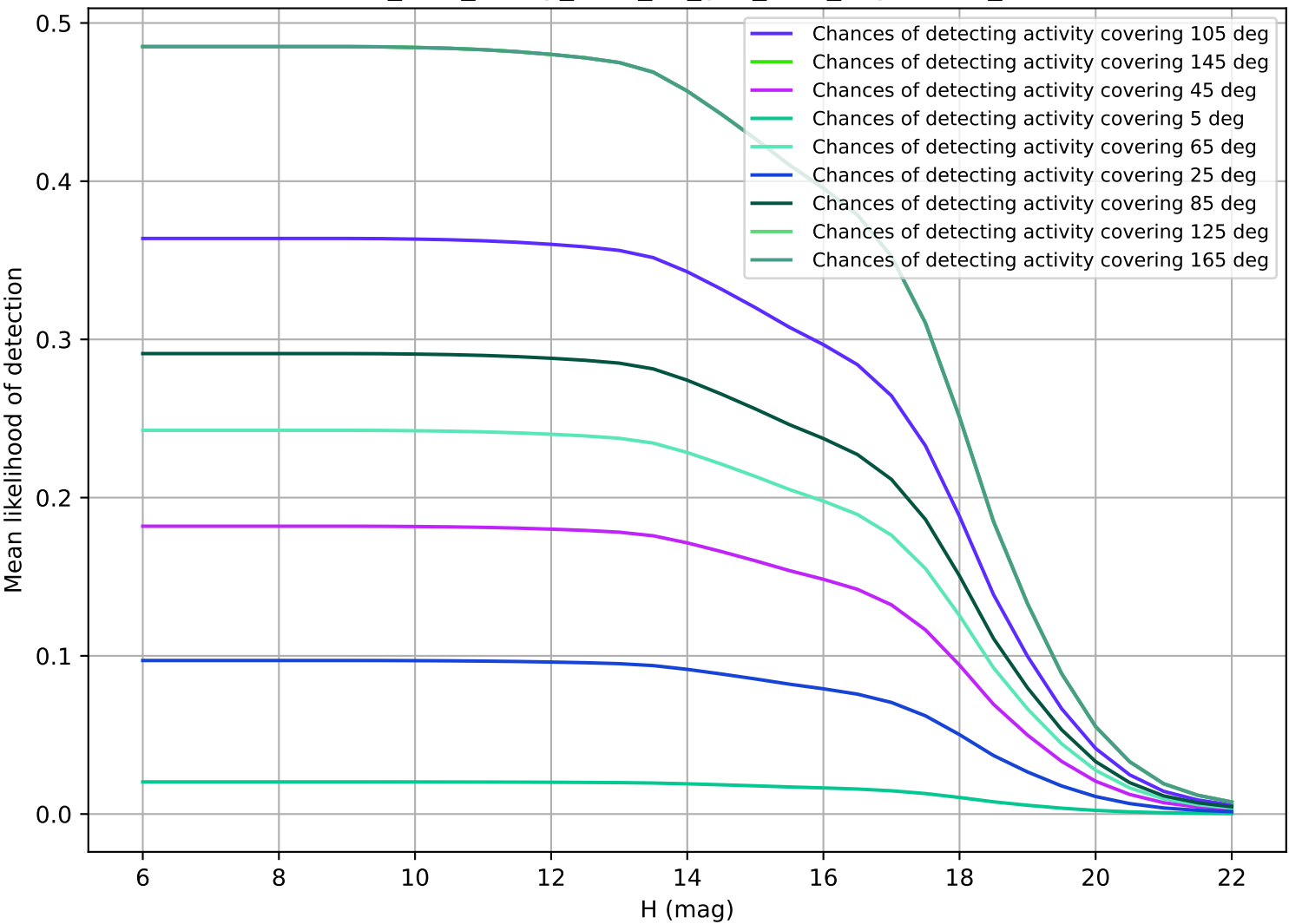
too_elab_heavy_r128_d3_griz_v3.4_10yrs OCC_r5
