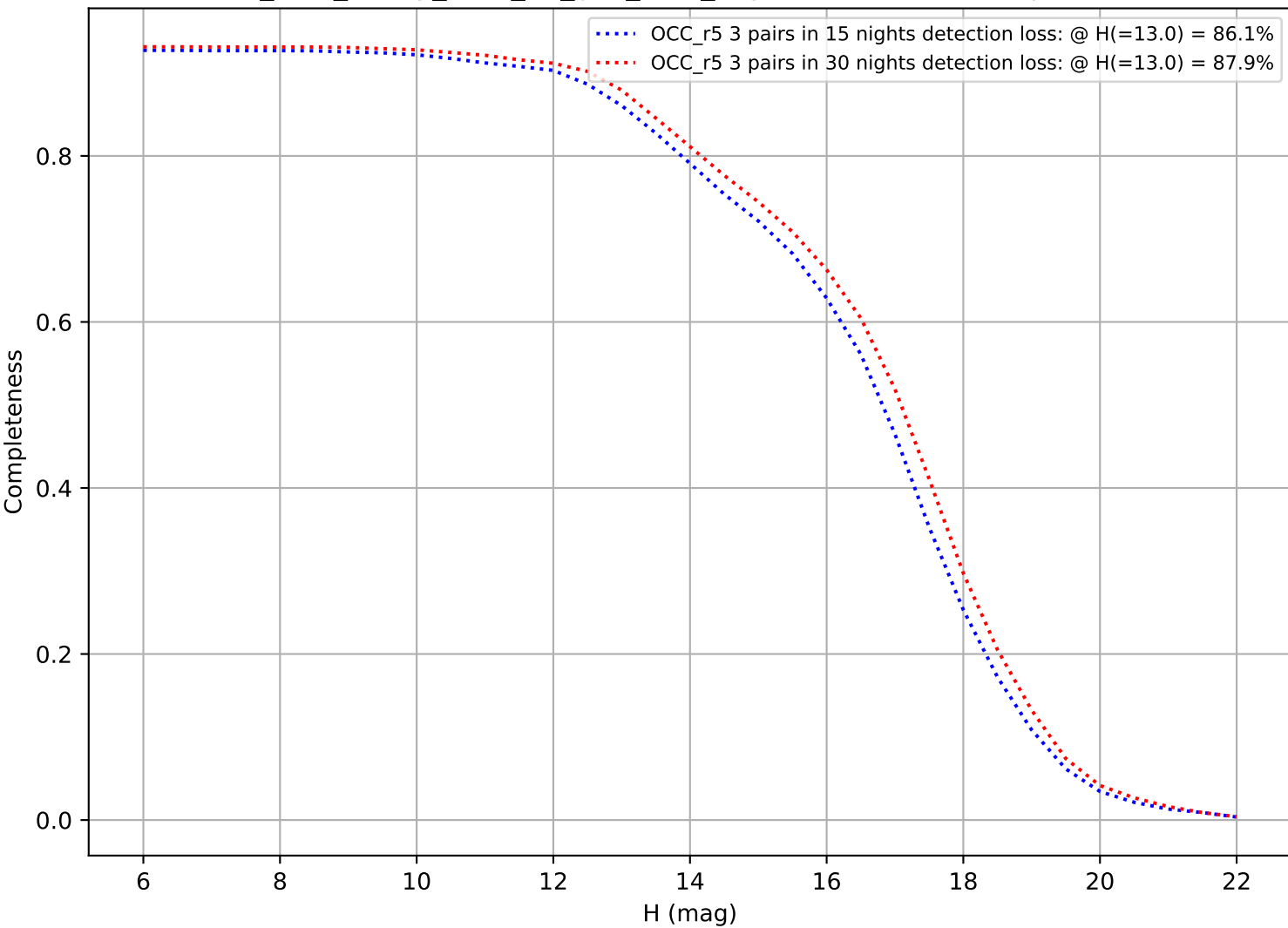
too_elab_heavy_r128_d3_griz_v3.4_10yrs: DifferentialCompleteness
