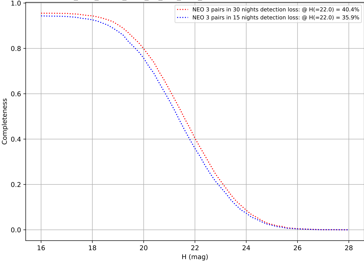
too_elab_heavy_r128_d3_griz_v3.4_10yrs: DifferentialCompleteness
