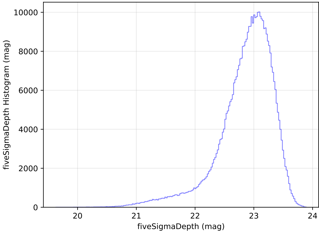
too_elab_heavy_r128_d3_griz_v3.4_10yrs z: fiveSigmaDepth Histogram
