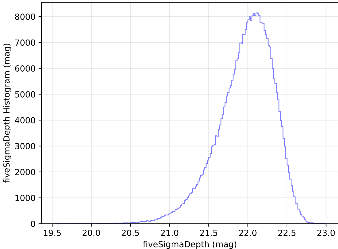
too_elab_heavy_r128_d3_griz_v3.4_10yrs y: fiveSigmaDepth Histogram
