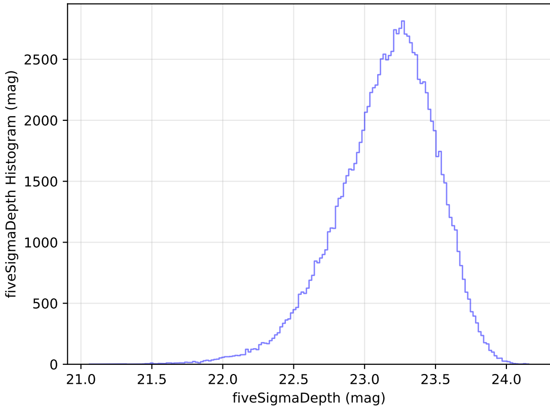
too_elab_heavy_r128_d3_griz_v3.4_10yrs u: fiveSigmaDepth Histogram
