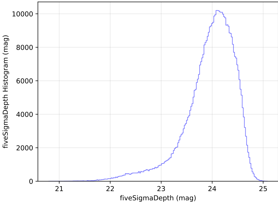
too_elab_heavy_r128_d3_griz_v3.4_10yrs r: fiveSigmaDepth Histogram
