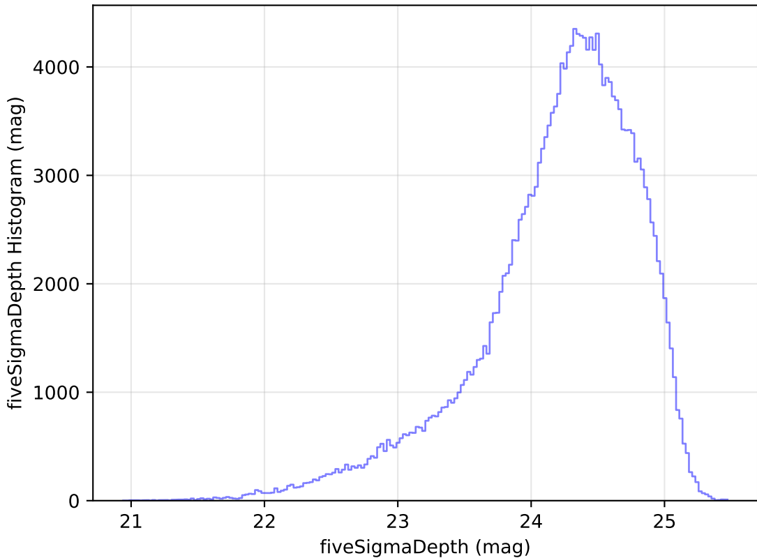
too_elab_heavy_r128_d3_griz_v3.4_10yrs g: fiveSigmaDepth Histogram
