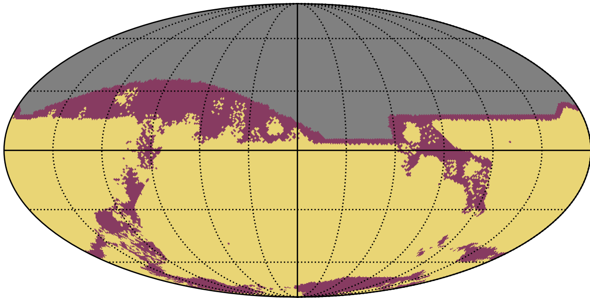
too_elab_heavy_r128_d3_griz_v3.4_10yrs : RapidRevisits
