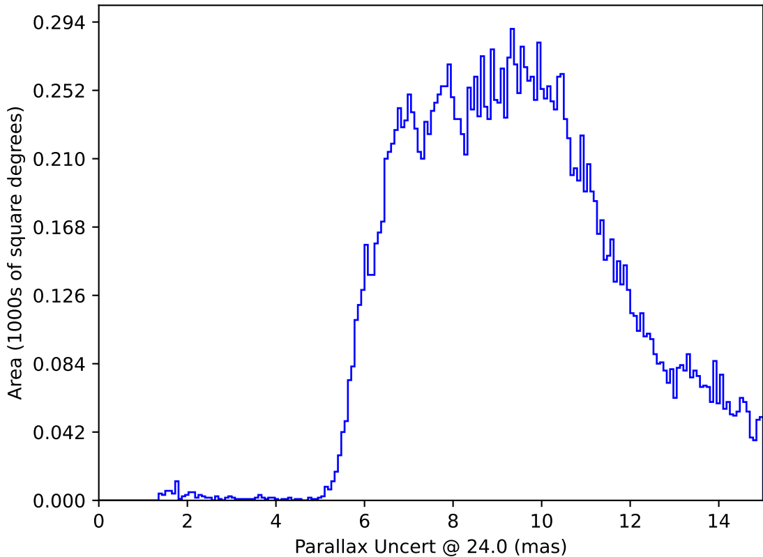
too_elab_heavy_r128_d3_griz_v3.4_10yrs : Parallax Uncert @ 24.0
