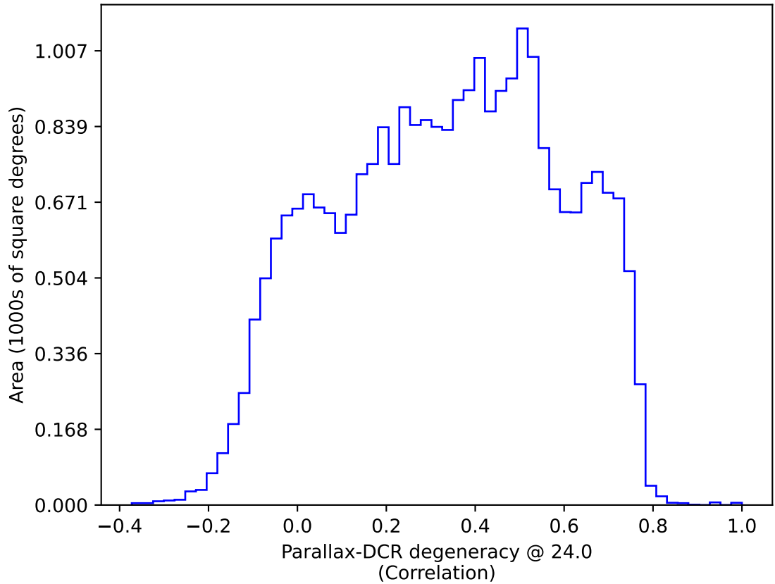
too_elab_heavy_r128_d3_griz_v3.4_10yrs : Parallax-DCR degeneracy @ 24.0
