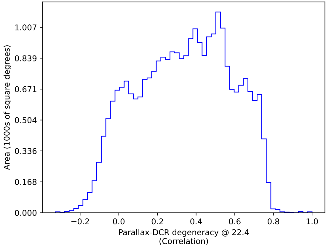
too_elab_heavy_r128_d3_griz_v3.4_10yrs : Parallax-DCR degeneracy @ 22.4
