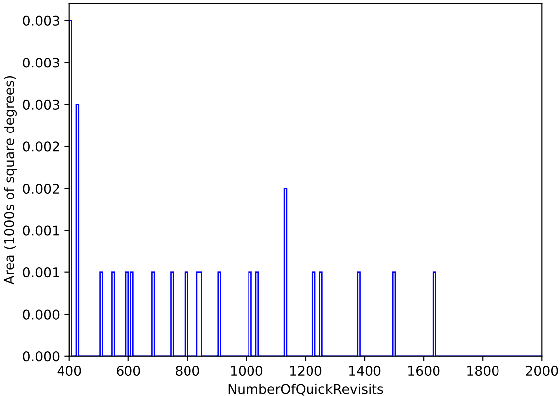
too_elab_heavy_r128_d3_griz_v3.4_10yrs : NumberOfQuickRevisits
