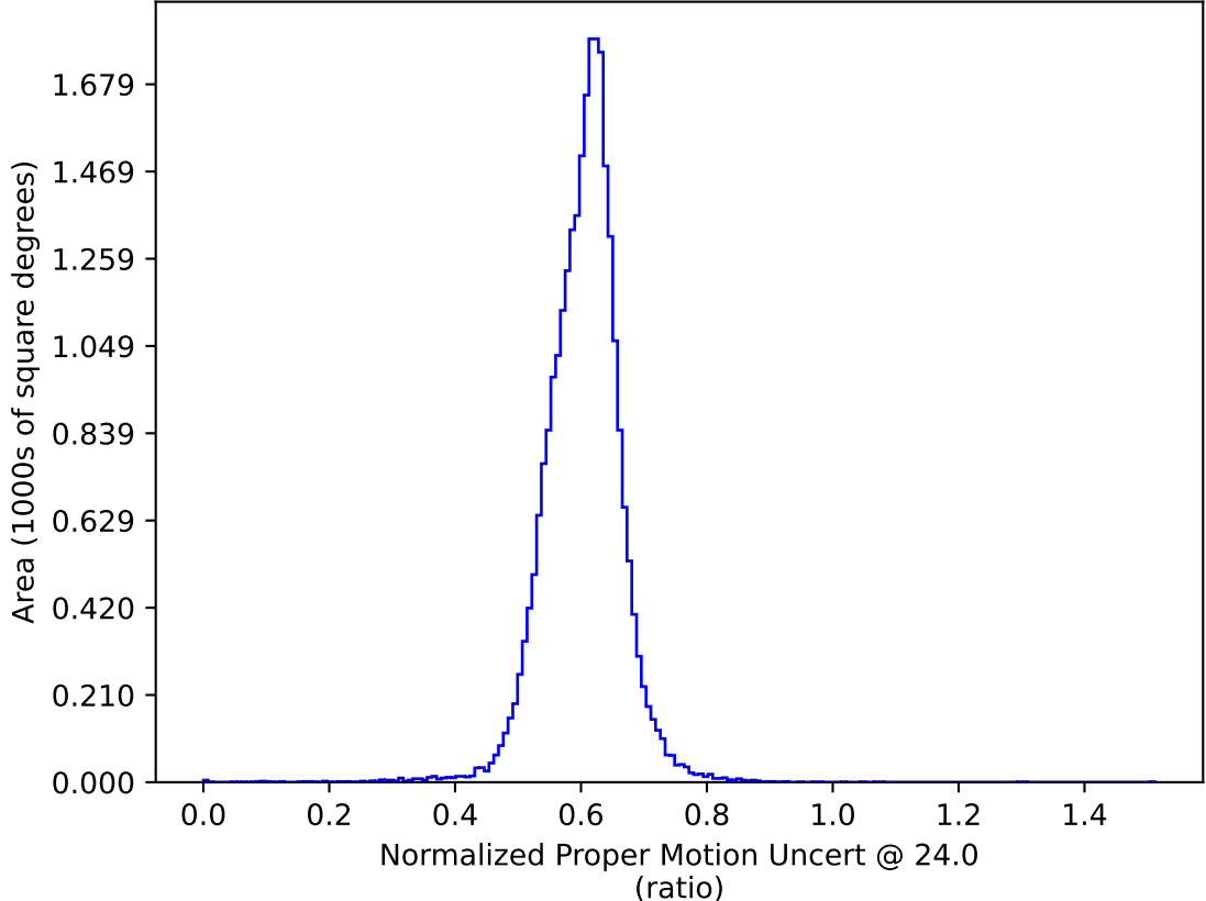
too_elab_heavy_r128_d3_griz_v3.4_10yrs : Normalized Proper Motion Uncert @ 24.0
