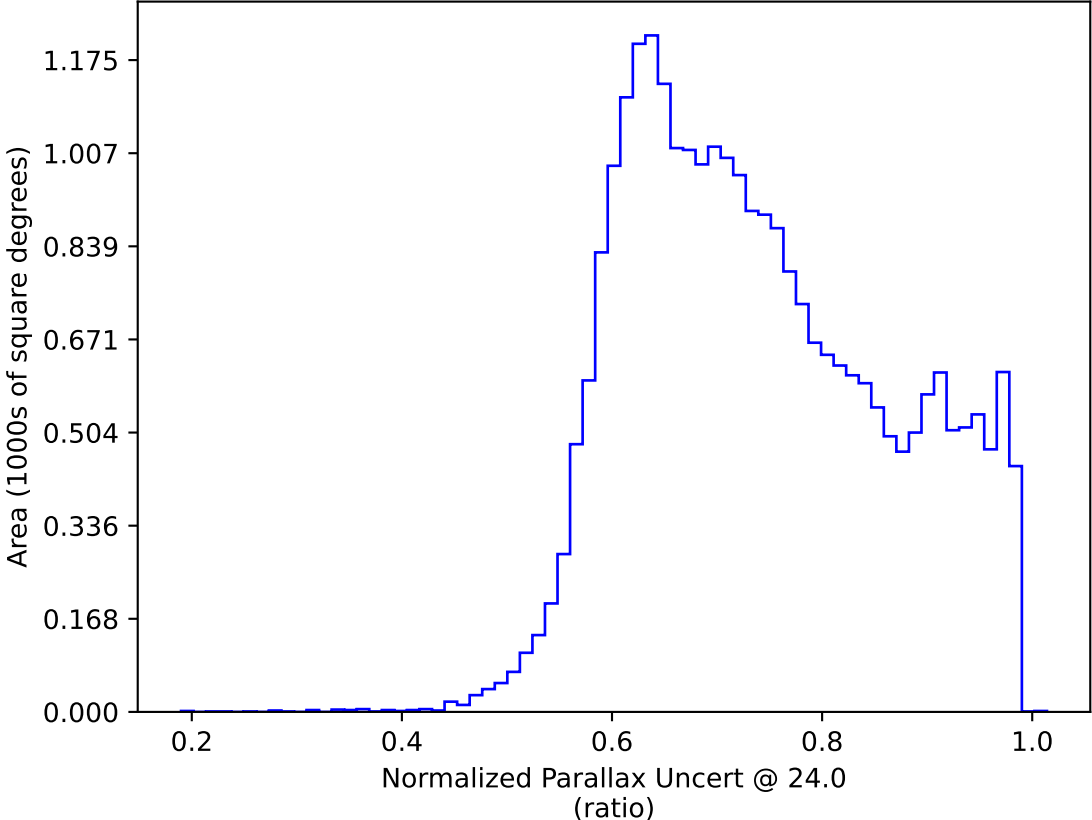
too_elab_heavy_r128_d3_griz_v3.4_10yrs : Normalized Parallax Uncert @ 24.0
