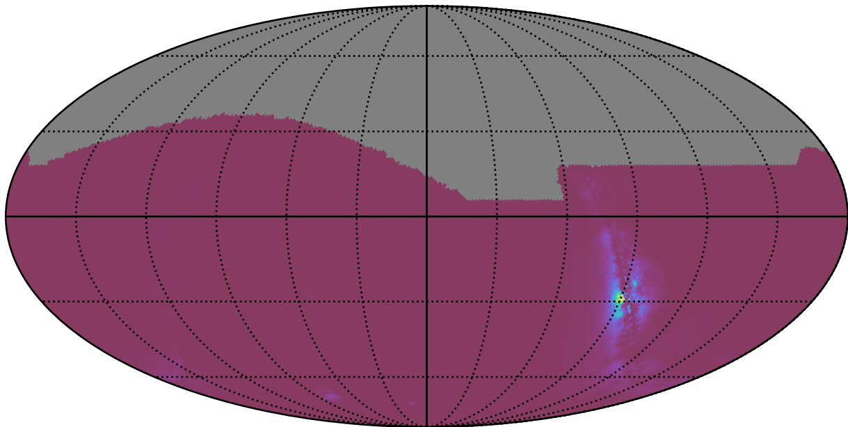
too_elab_heavy_r128_d3_griz_v3.4_10yrs : NlcPoints
