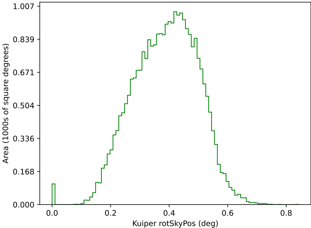
too_elab_heavy_r128_d3_griz_v3.4_10yrs g: Kuiper rotSkyPos
