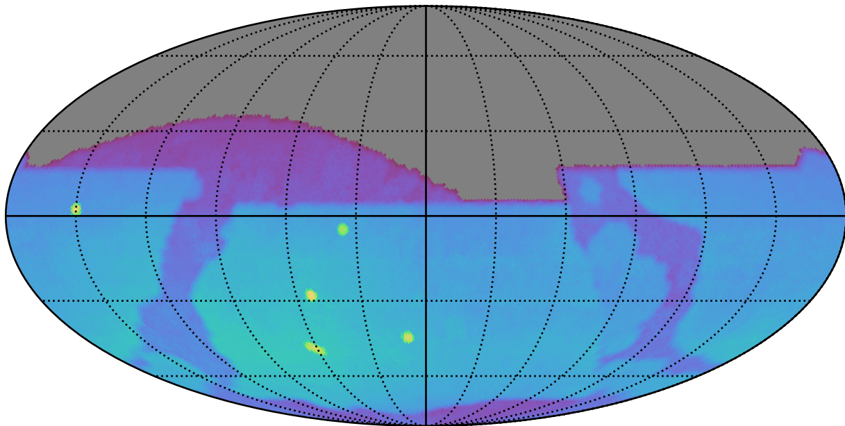
too_elab_heavy_r128_d3_griz_v3.4_10yrs : Brown Dwarf, L4
